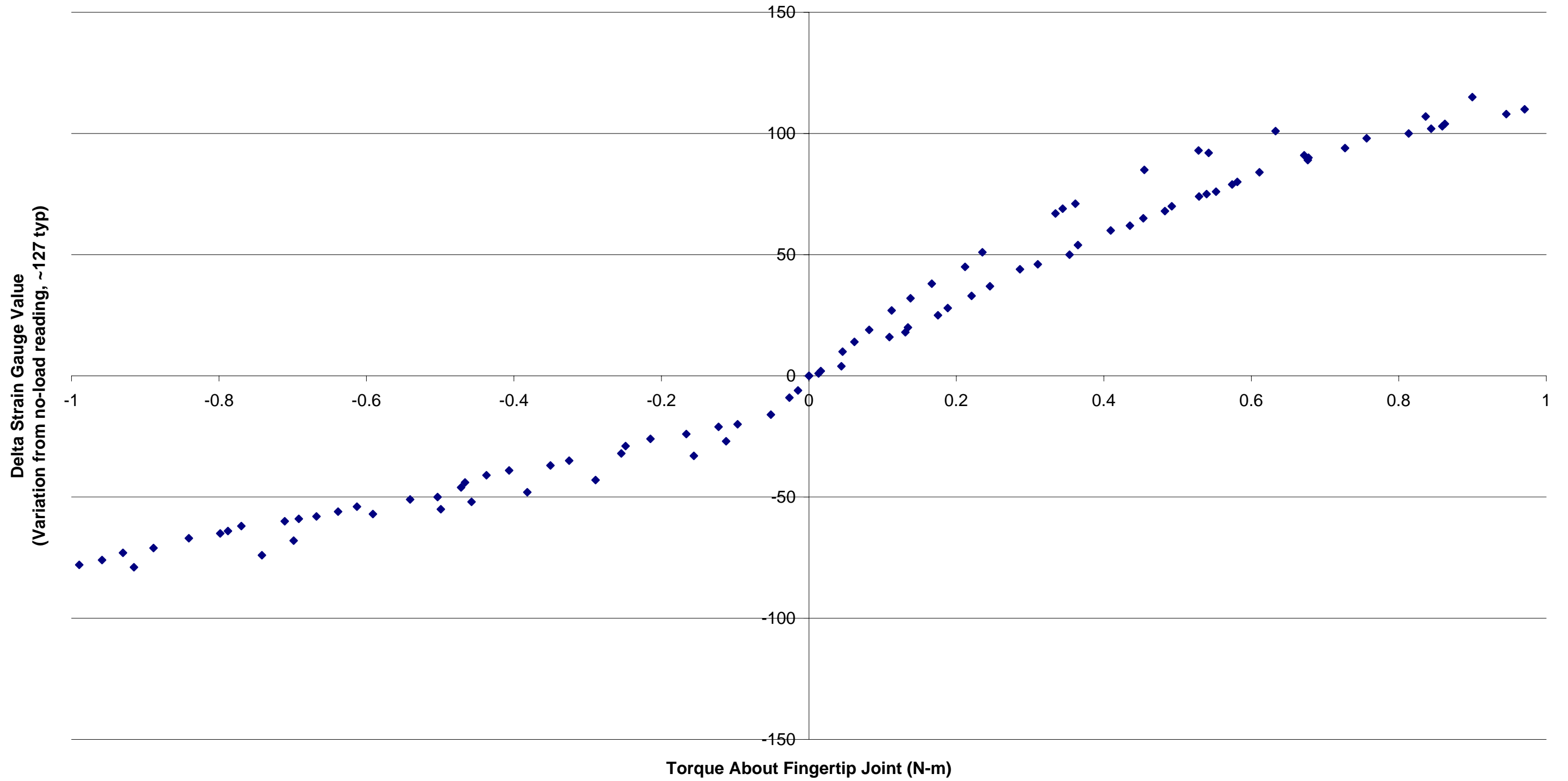
Torque Vs. Delta Strain Gauge values (includes hysteresis)
