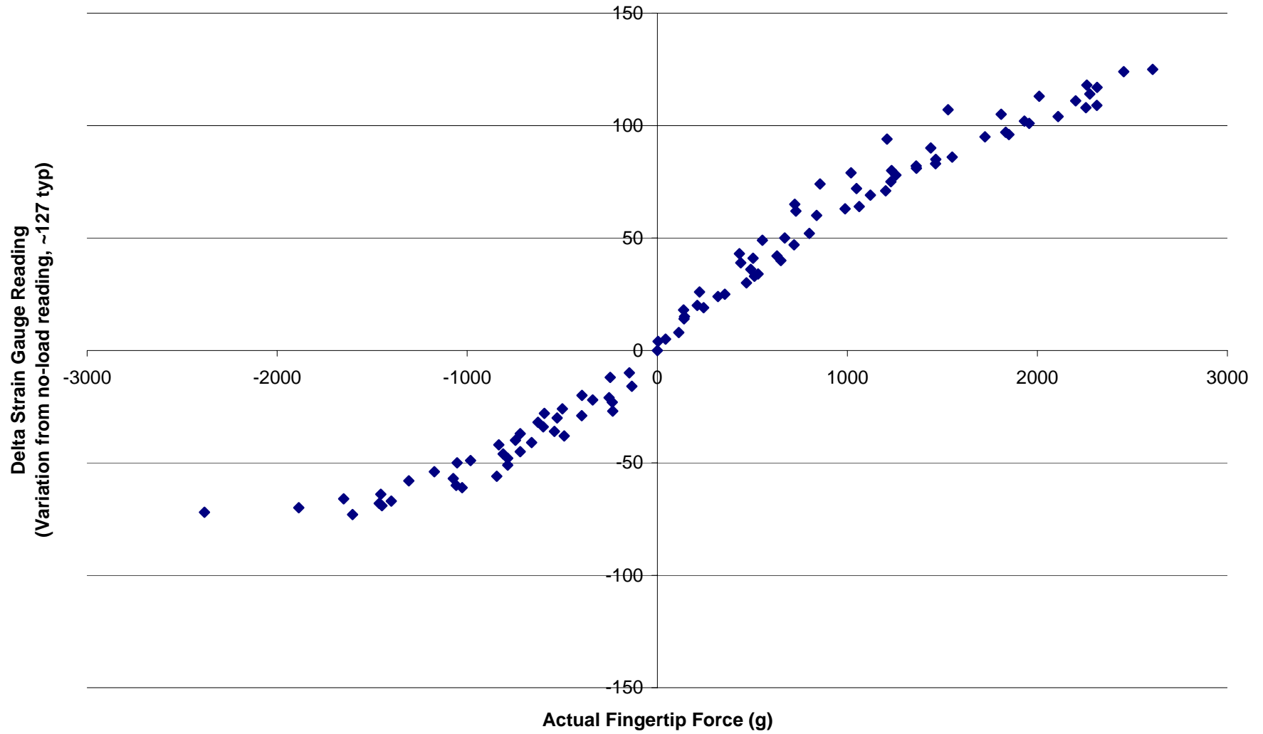
Actual Force Vs. Delta Strain Gauge Reading (includes hysteresis)
