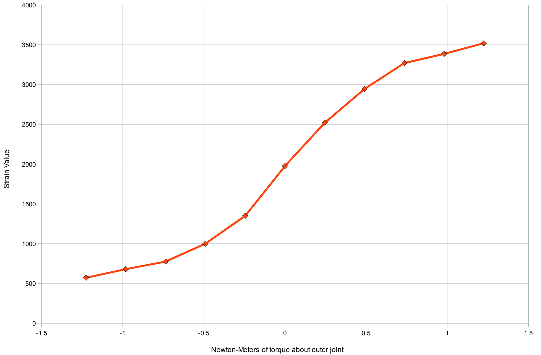
BH8-280 Strain Gage Calibration
